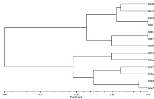
Figure 4. Dendrogram of 13 accessions of jatropha plant cluster analysis using UPGMA based on RAPD banding pattern using 10 primer
