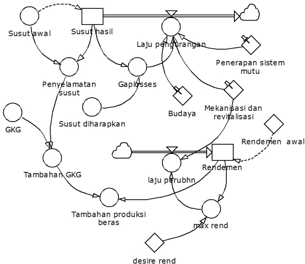
Gambar 4. Diagram stock flow sub sistem susut padi
