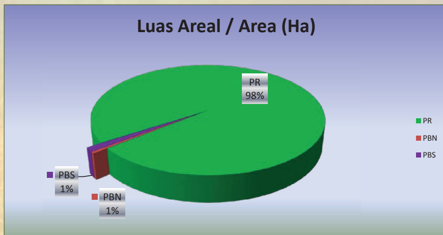
Figure Area and Production Comparison Graph of Clove by Farming Category, 2016
