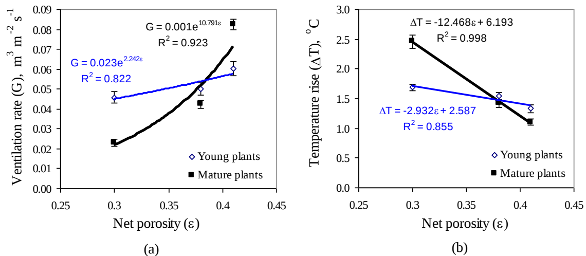
Figure 3. The relationships between (A) net porosity and ventilation rate and (B) net porosity and temperature rise in tropical greenhouses; R^2 , coefficient of determination.
