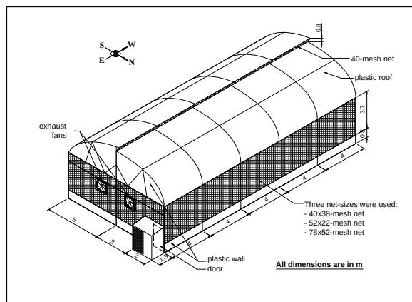
Figure 1. Isometric View of The Adapted Greenhouse Structure Used for The Experiment.
