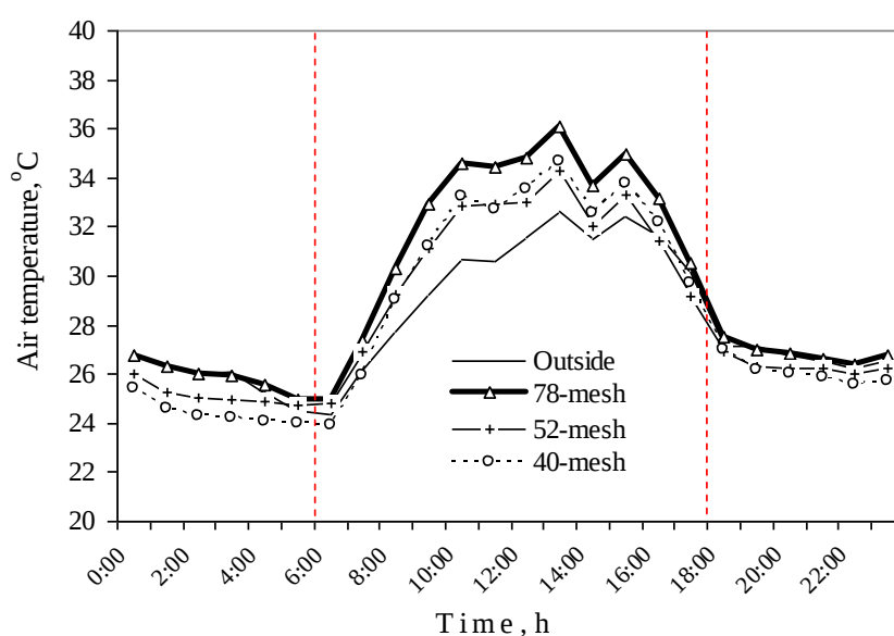
Figure 2. Diurnal air temperature in each greenhouse and ambient for the typical day.
