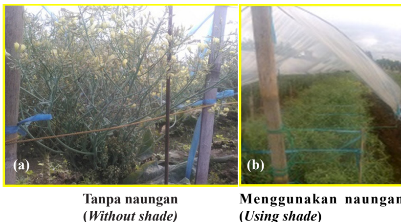
Gambar 2. Tanaman perbenihan kubis bunga tanpa naungan (a) dan menggunakan naungan (b) [Cauliflower seed without shade (a) and using shade (b)]
